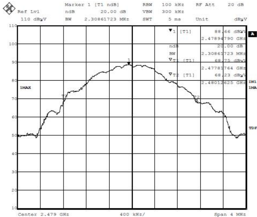
High Channel – Bandwidth 2.309 MHz
