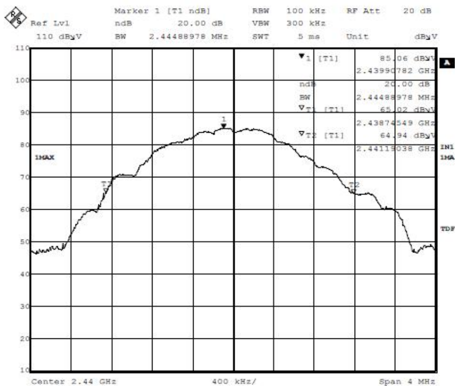
Mid Channel – Bandwidth 2.448MHz
