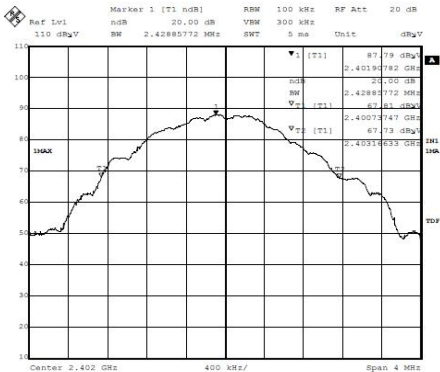
Low Channel – Bandwidth 2.429MHz
